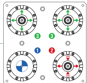
拉栓安裝示意圖 Pull-bolt mounting schematic
